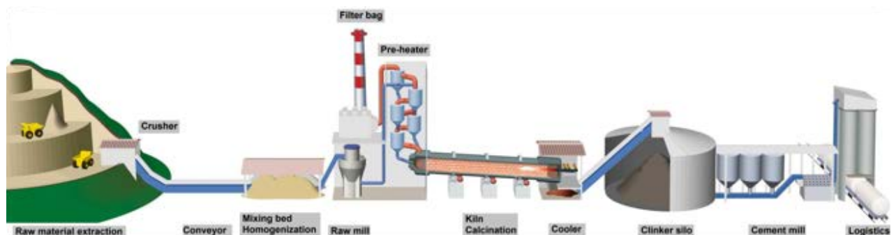
■ Typical cement manufacturing process (Courtesy: Holcim)
