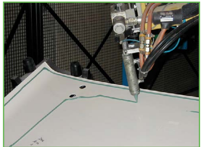
■ Adhesive application by robot
